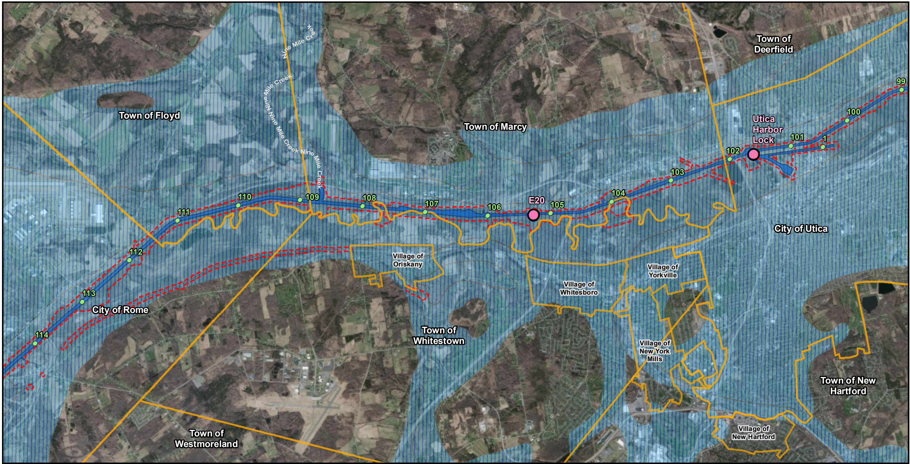
Figure 47F: Aquifers
